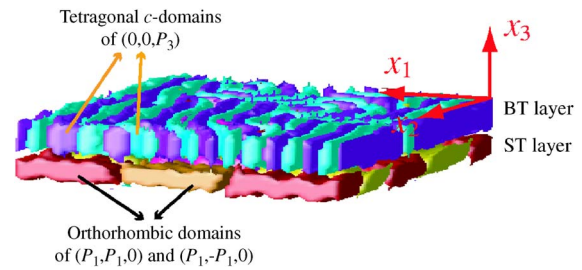
FIG. 2. (Color online) Domain morphology of a fully relaxed superlattice of \text{ST}_4/\text{BT}_8 at room temperature.
